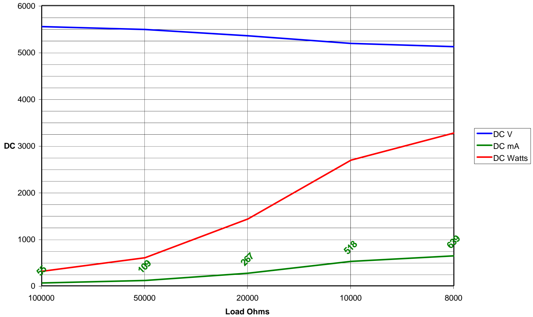
Series Secondaries, C filter, 0-3KW DC
