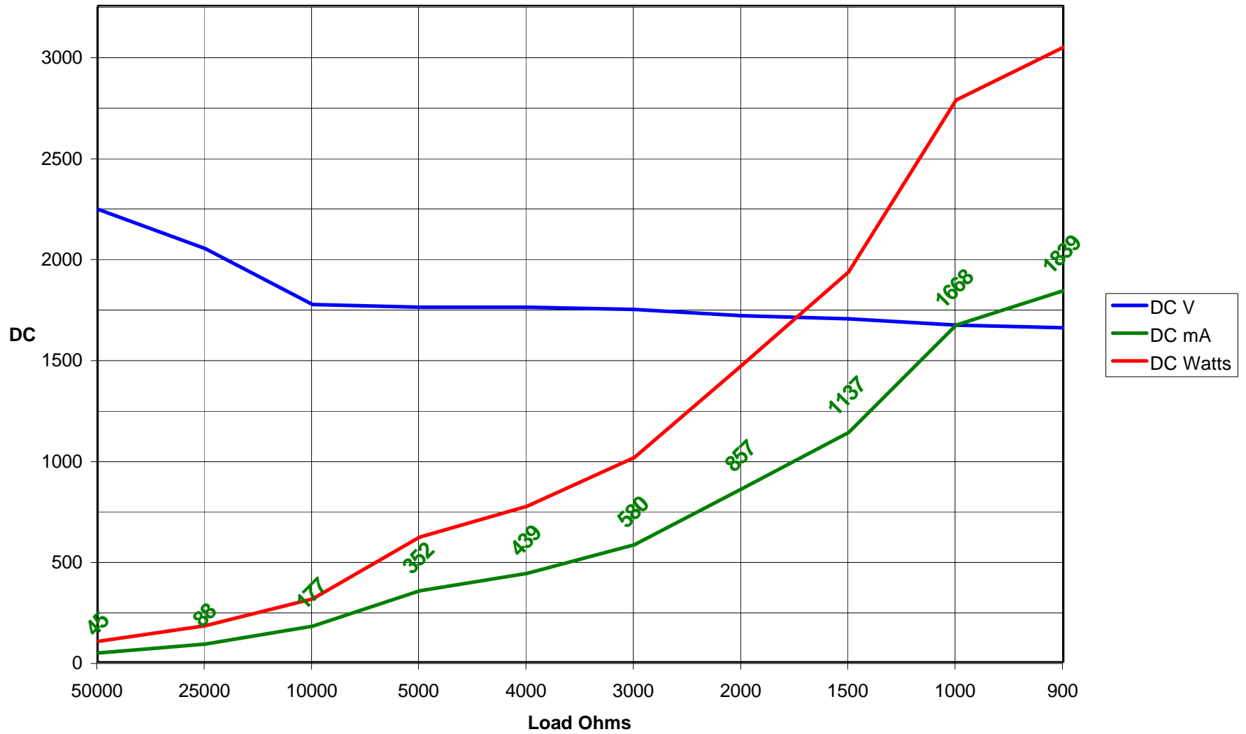
Parallel Secondaries, LC filter, 0-3KW DC
