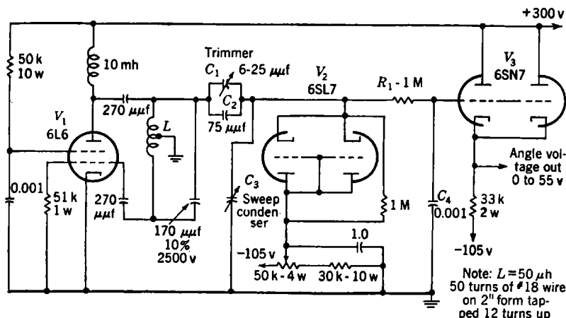
FIG. 5-37.—Angle-voltage generator.
