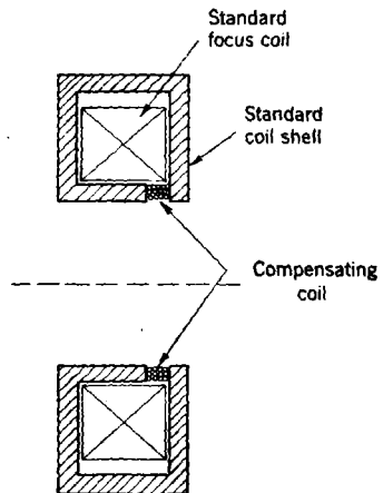
FIG. 3-13.—Focus coil for focus compensation with deflection.
