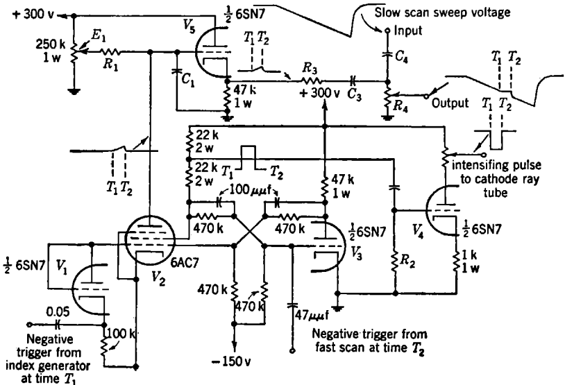
FIG. 6-8.—Sweep-stopping circuit.
