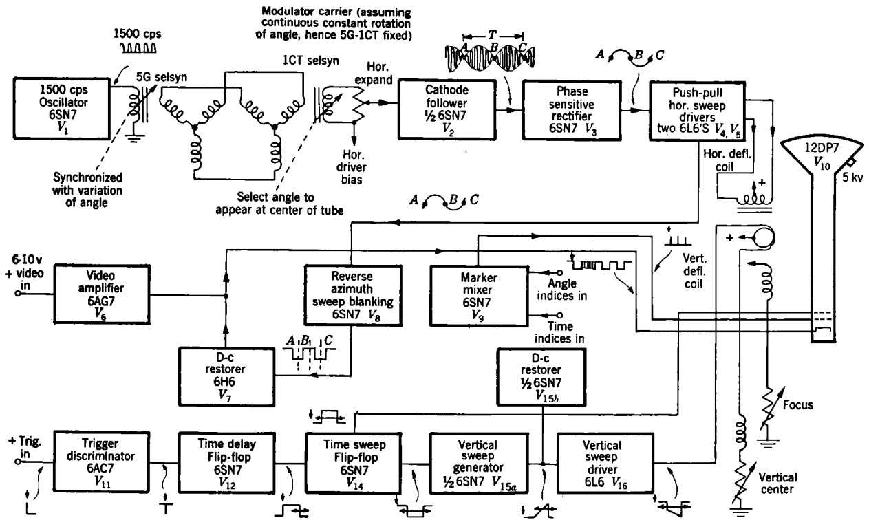
FIG. 11-6.—Block diagram, B-scan.
