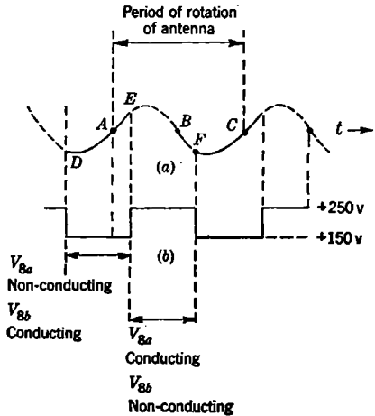
FIG. 11-8.—Method of blanking return azimuth sweep in a B-scan. (a) Azimuth voltage sine wave applied to grid of azimuth sweep-blanking tube V_{8a} . (b) Square-wave blanking pulse on plate of V_{8a} , which is used to blank the cathode-ray tube during the positive interval, EF , corresponding to the time of the reverse sweep control about B . Dashed portion of (a) represents reverse azimuth sweep.
