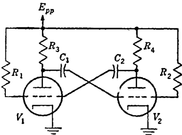
FIG. 4-22.—Multivibrator circuit.
