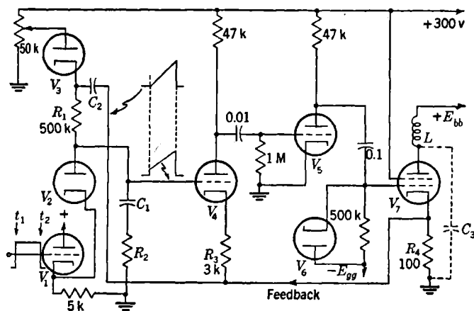
FIG. 10-7.—Three-stage feedback amplifier.
