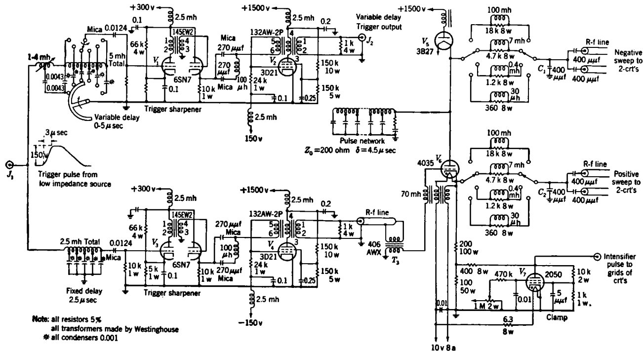
FIG. 7-26.—Schematic diagram of high-speed synchroscope.
