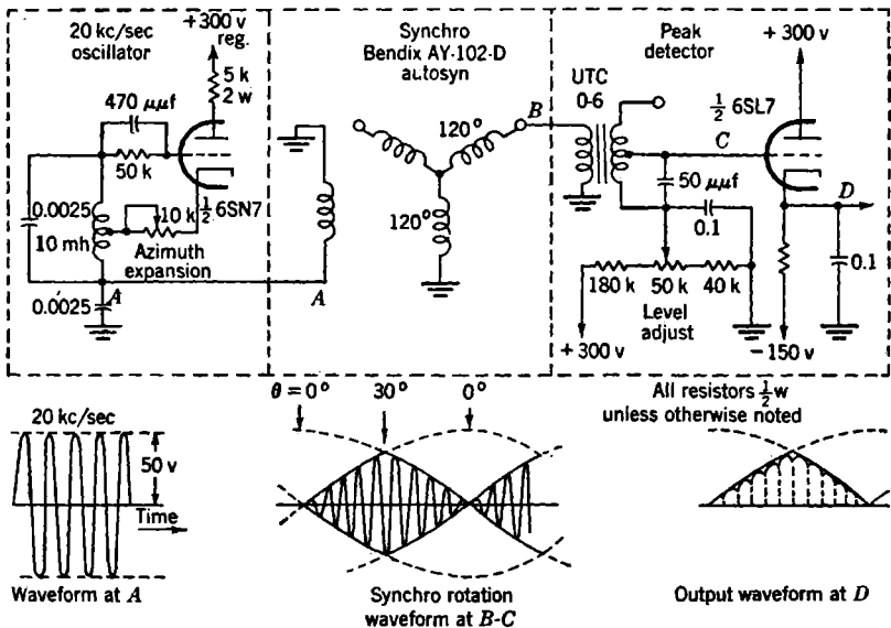
FIG. 5-31.—Synchro data transmission for 30^\circ quadrant.
