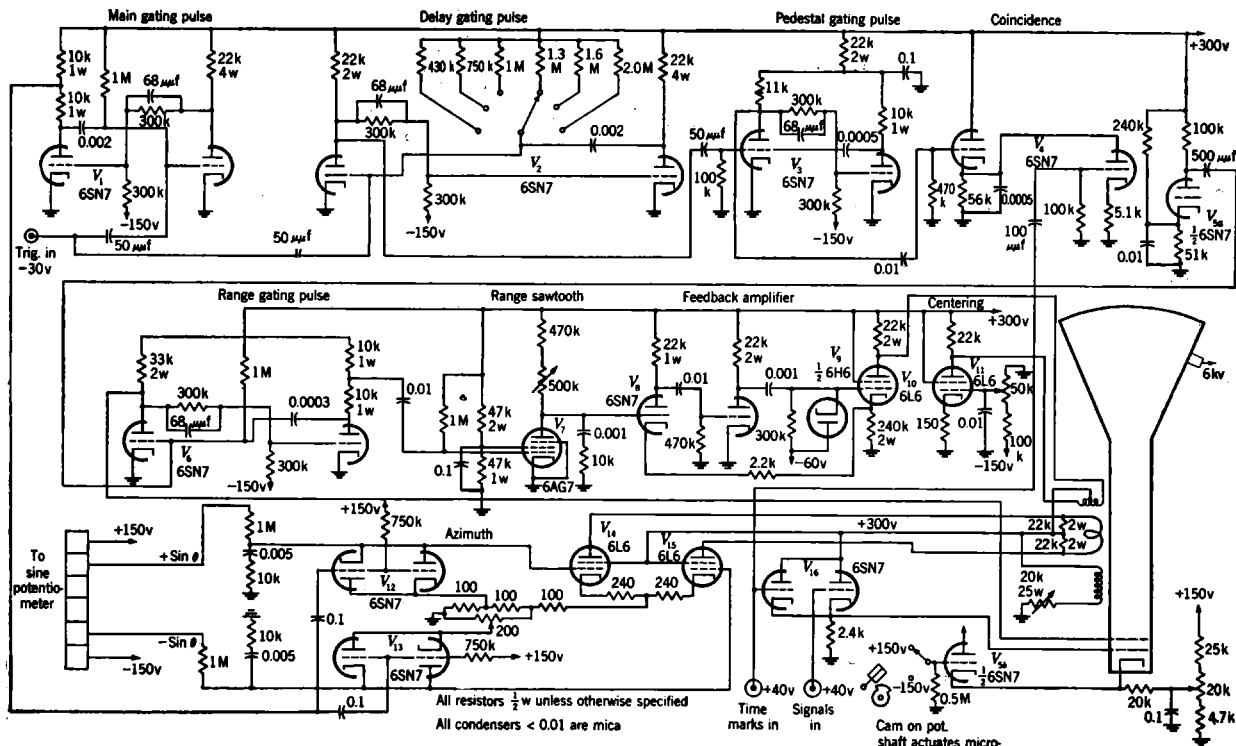
FIG. 14-18.—Electrical schematic diagram for sector produced by two time bases.
