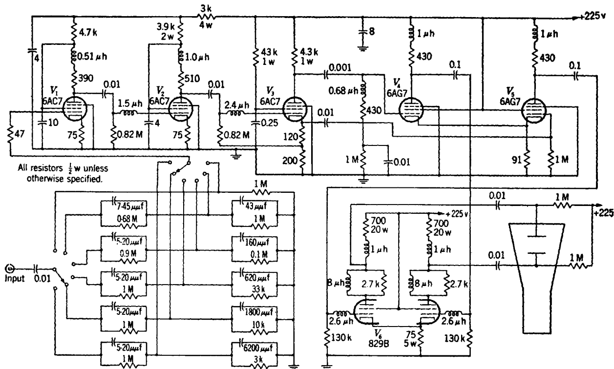
FIG. 7-10.—Schematic diagram of wideband video amplifier for Model 5 synchroscope.
