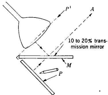
FIG. 16-20.—Method of superposing maps or plots on a CRT.
