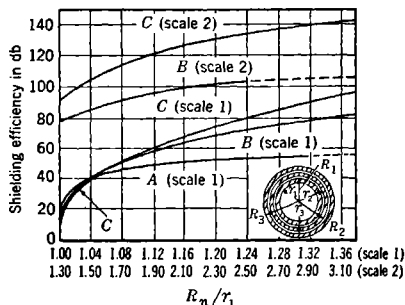
FIG. 16-13.—Shielding efficiency of one, two, and three concentric cylinders (for zero frequency). Shielding efficiency = 20 \log_{10} H_e/H_s , where H_e = field intensity without shield, and H_s = field intensity with shield. \mu = 5000 , R_1/r_1 = r_2/R_1 = R_2/r_2 = r_3/R_2 = R_3/r_3 . Curve A—one cylinder R_n/r_1 = R_1/r_1 ; Curve B—two cylinders R_n/r_1 = R_2/R_1 ; Curve C—three cylinders R_n/r_1 = R_3/r_1 . Cylinders considered infinitely long. Direction of flux perpendicular to axis of cylinders. (Courtesy of Bell System Technical Journal.)
