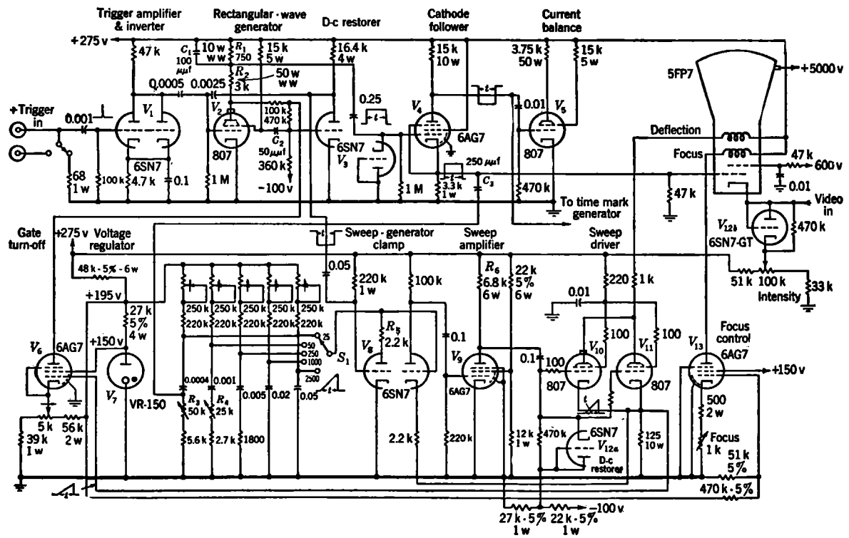
FIG. 13-5.—Rotating-coil radial-time-base display with current feedback.
