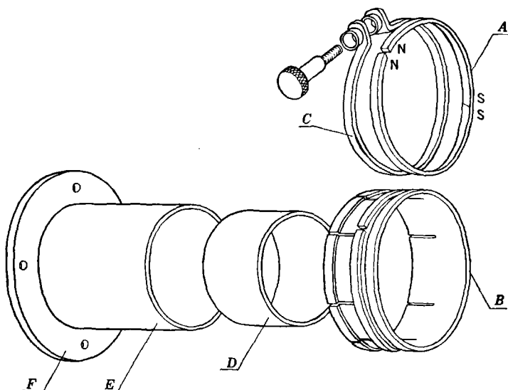
FIG. 9-5.—Precentering assembly. A , the magnet—GE “Cunife” alloy 0.120 × 0.050 strip, rolled into 2-in. ID circle; B , brass ring; C , brass clamping ring; D , soft iron shunt to be soldered into rear end of supporting cylinder; E , brass supporting cylinder; F , mounting flange.
