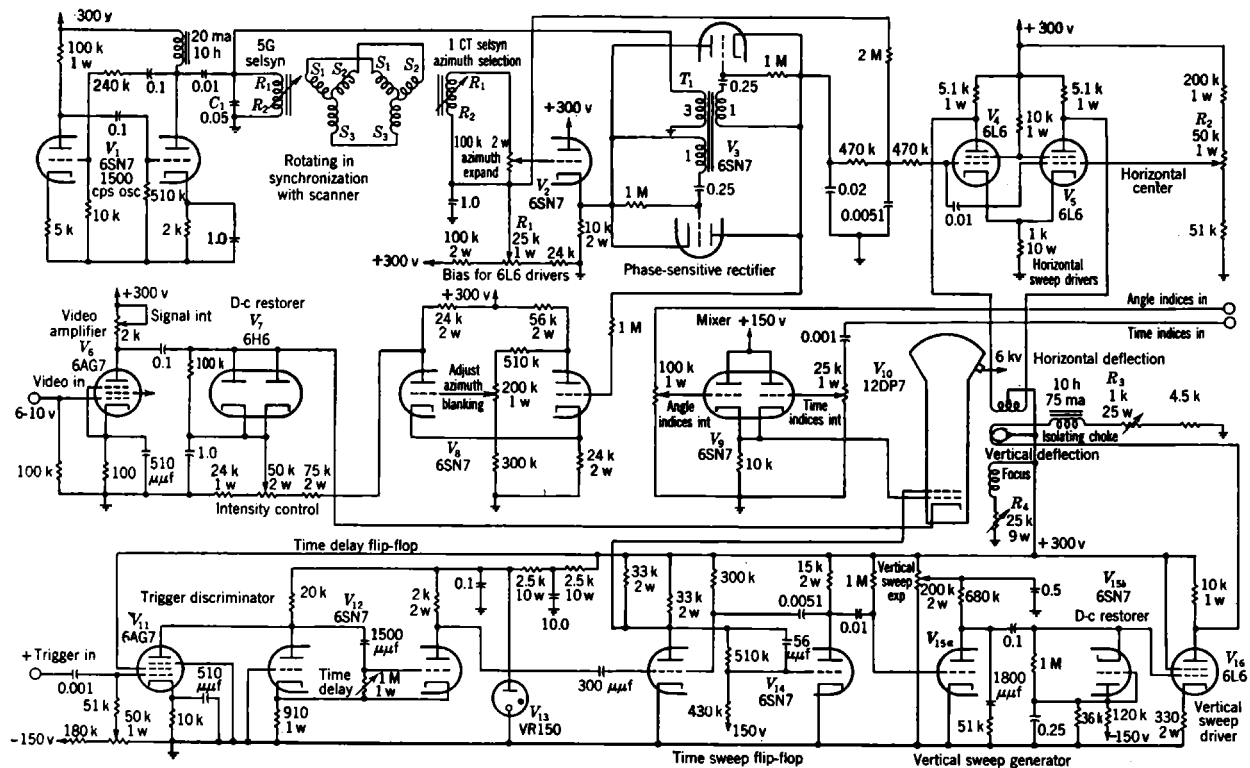
Fig. 11-7.—Circuit diagram, B-scan.
