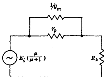
FIG. 4-11.—Equivalent circuit of cathode follower.
