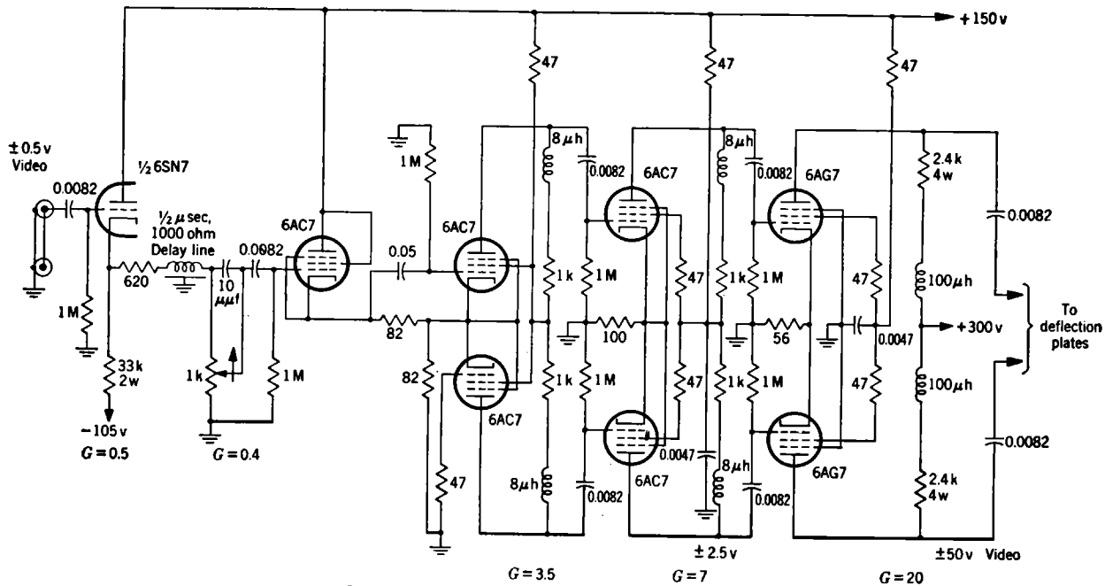
FIG. E-8.—Push-pull output with single-ended input.
