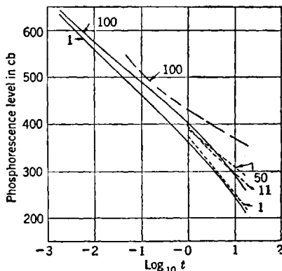
FIG. 18-40.—Comparison of phosphorescent decay from selected cascade and single layer screens. Time t in seconds.
