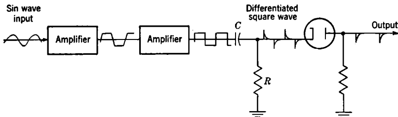
FIG. 4-18.—Deriving a trigger pulse from a sine wave.
