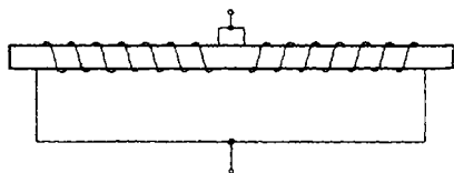
FIG. 8-12.—Balanced winding.
