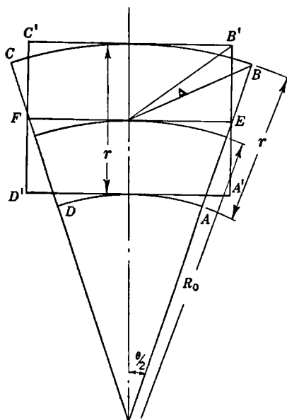
FIG. 14-6.—Geometry of range-normalized Micro-B sector.
