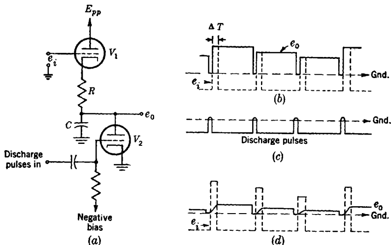
FIG. 5-17.—The boxcar demodulator. (a) Circuit schematic diagram. (b) Input and output waveforms for the case where (R + R_{KF})C \ll \Delta T , ( R_{KF} being resistance of the cathode follower) the peak-pulse amplitude determines the amplitude of the associated "boxcar" waveform. In the case where (R + R_{KF})C \gg \Delta T (Fig. 5-17d) it is the area of the pulse lying above the cutoff potential of V_1 which determines the boxcar amplitude. The chief advantage of the method lies in the fact that, except for the gaps between boxcars, the output amplitude has a magnitude determined by the latest available information and that it can follow a rapid rate of change of pulse amplitude. The amount of carrier-frequency component due to the gaps between the boxcars is appreciable, but for many appli-
