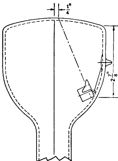
Fig. 18-65 —Evaporator mounting.
