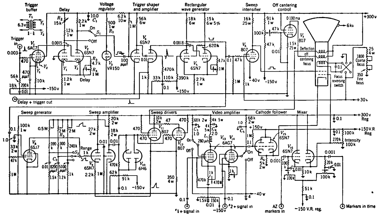
Fig. 13-6.—Rotating-coil radial-time-base display with off-centering.
