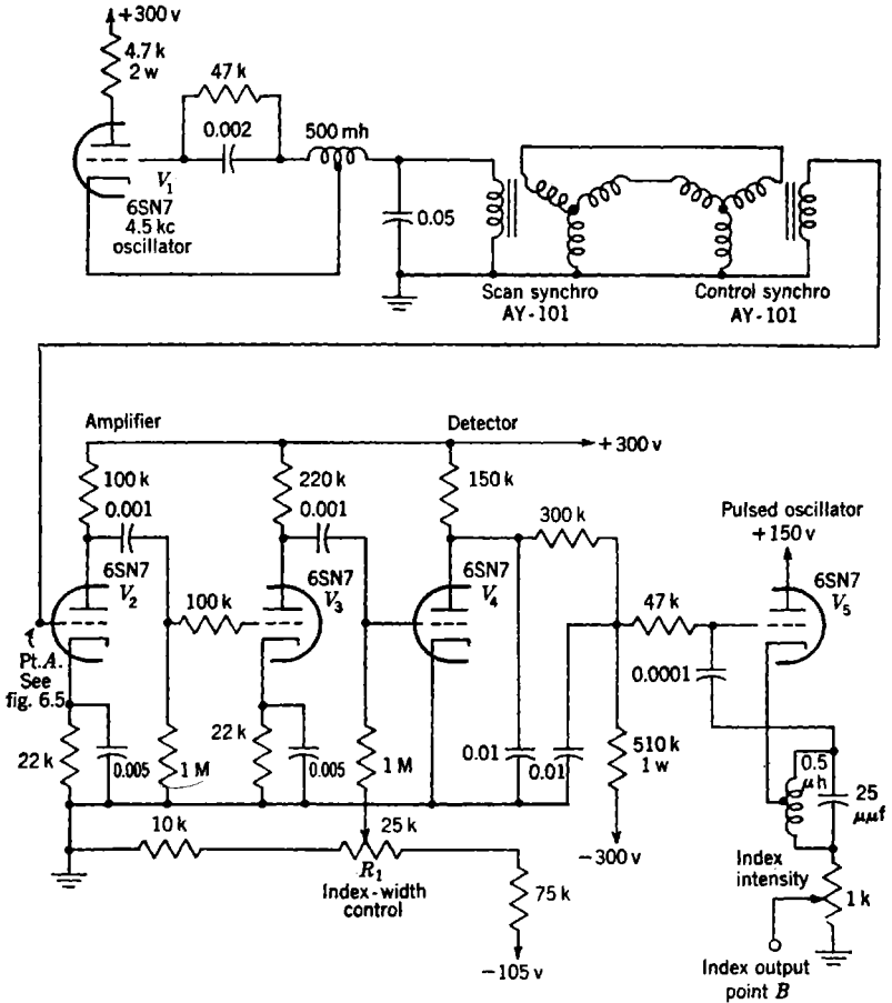
FIG. 6-4.—Synchro-null indices.
