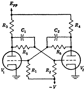
FIG. 4-24.—Scale-of-two circuit.
