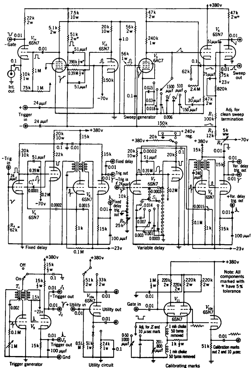
FIG. 7-14.—Schematic circuit diagram of Model G synchronizer.
