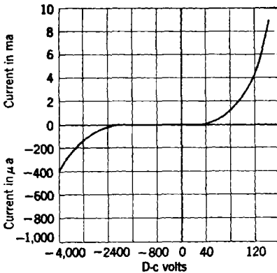
FIG. 4-72.—Selenium-rectifier characteristic, 110-disk-assembly high-temperature type.
