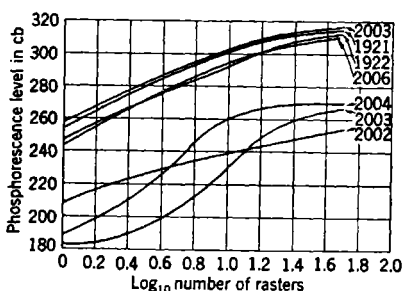
FIG. 18-15.—Buildup under repeated electron excitation. Screen excited at 10-sec intervals with observations 10 sec after each excitation. Q = 20 \text{ } \mu\text{mc}/\text{cm}^2 per raster. See Table 18-1 for screen compositions.
