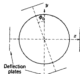
FIG. 7-29.—Nonorthogonality of deflection plates.
