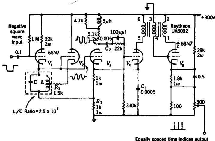
FIG. 6-15.—Generator of multiple time indices.
