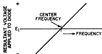
Fig. 32—Diagram showing resultant voltage E_r in Fig. 31 as a function of frequency.
