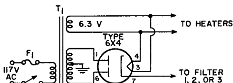
POWER SUPPLY 2
