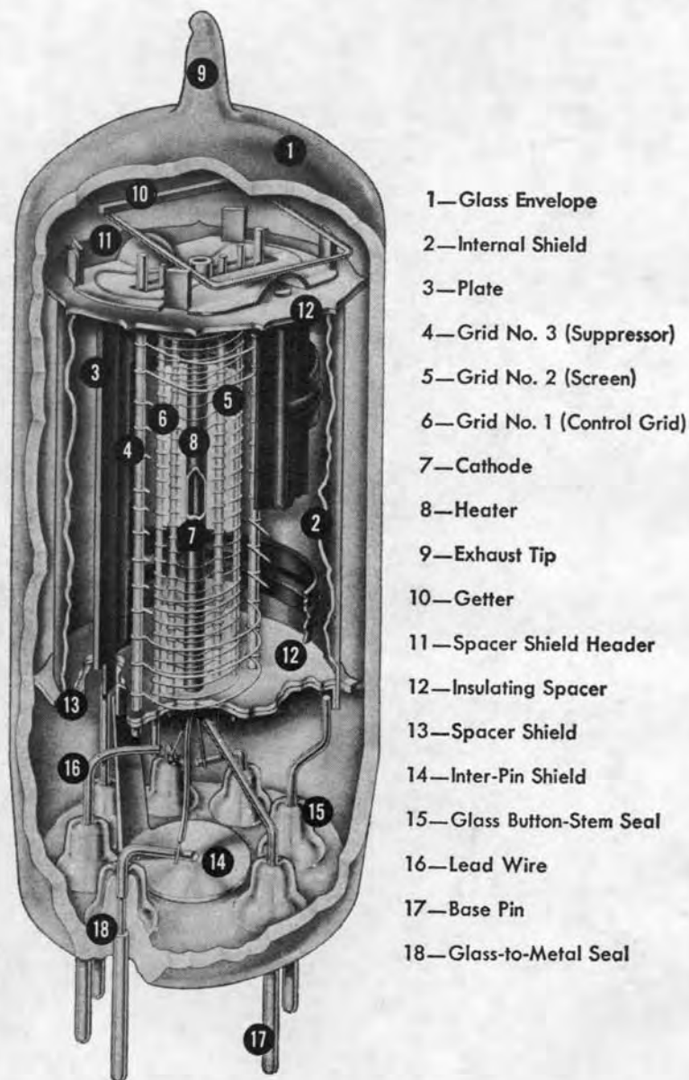
Structure of a Miniature Tube
